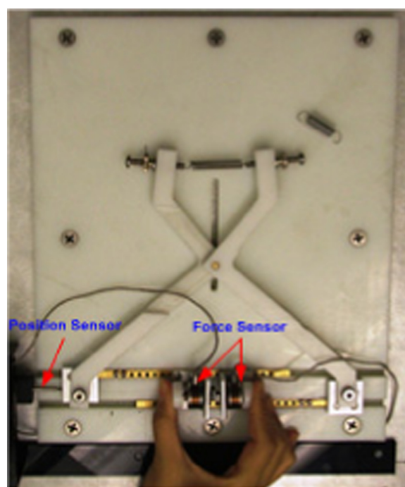
Figure 1. Self-made device for finger grip. Two force sensors were mounted on the end of two sliding tracks. One position sensor measured the displacement when gripping. The force produced by the thumb and index finger were recorded and fed back to the subject in the visual paradigm.
